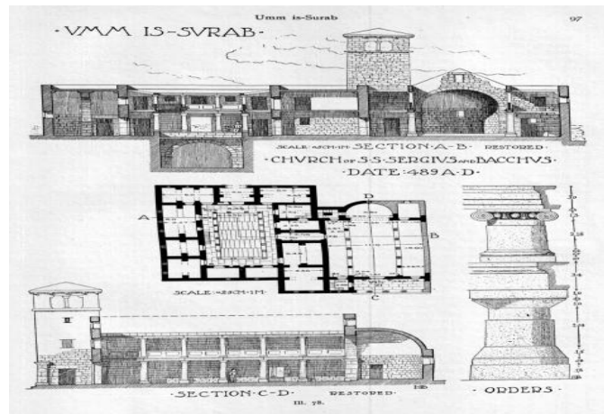
Graphic documentation of the Church of Saints Sergius and Bacchus at Umm al-Surab by H. C. Butler, after Butler 1919, ill. 78, p. 97
